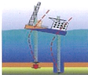
Punch Through during Installation
