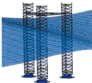
Jackup-wave-soil interaction
